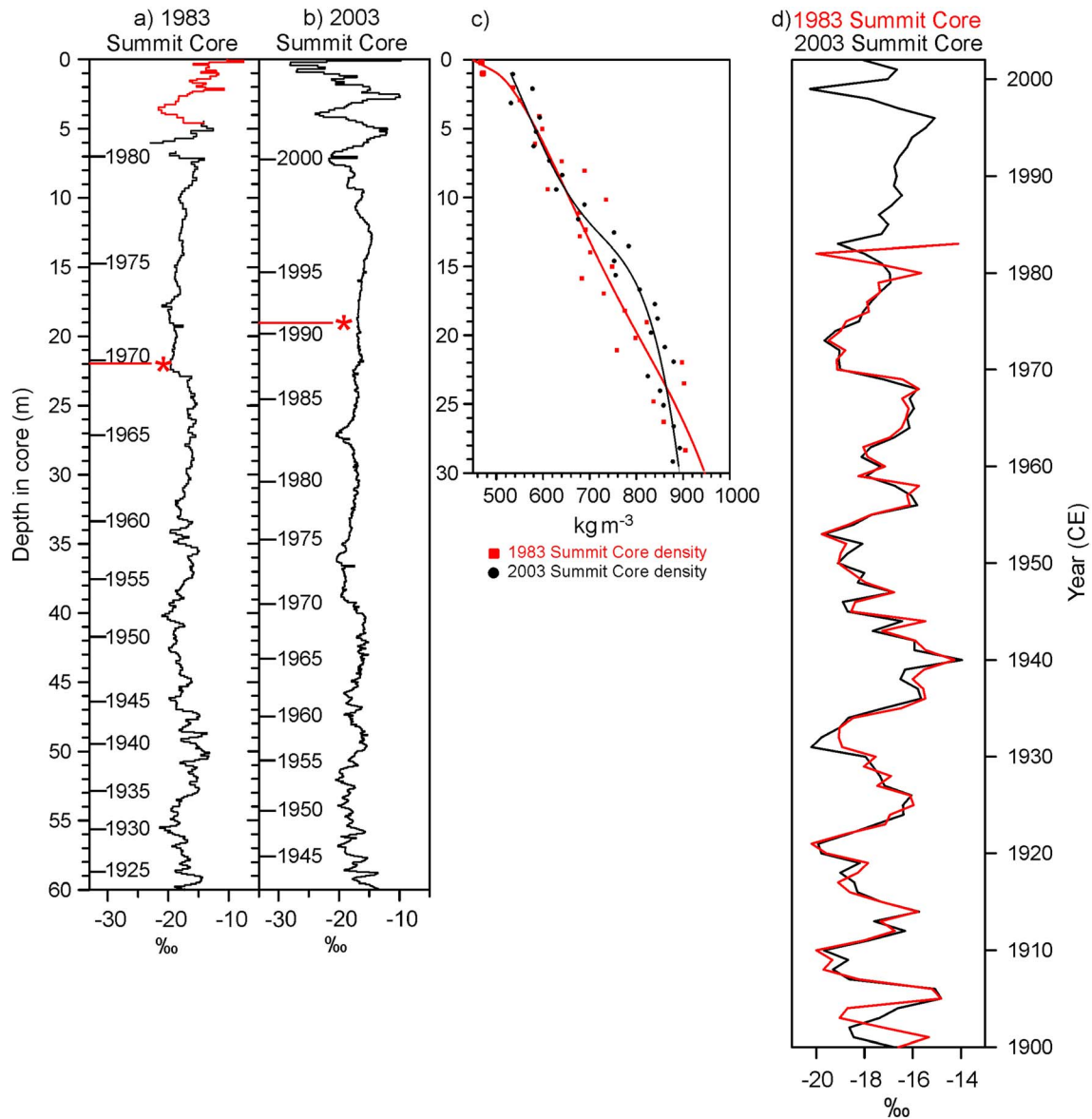
Figure 3. \delta^{18}\text{O} stratigraphy in the top 60 m of (a) the 1983 QIC summit core (dated back to TY1925) topped by a 2.5 m pit and part of the summit shallow core (red curve) and (b) the 2003 QIC summit dome core (dated back to TY1945). The pore close-off density of 830\text{ kg m}^{-3} is marked by a red line and asterisk in each profile. (c) The density profiles to 30 m of both records are aligned by depth with the \delta^{18}\text{O} plots. Each plot is overlain by a fourth-order regression curve. (d) Annual averages of \delta^{18}\text{O} through the twentieth century for the 1983 (red curve) and the 2003 summit (black curve) cores.
