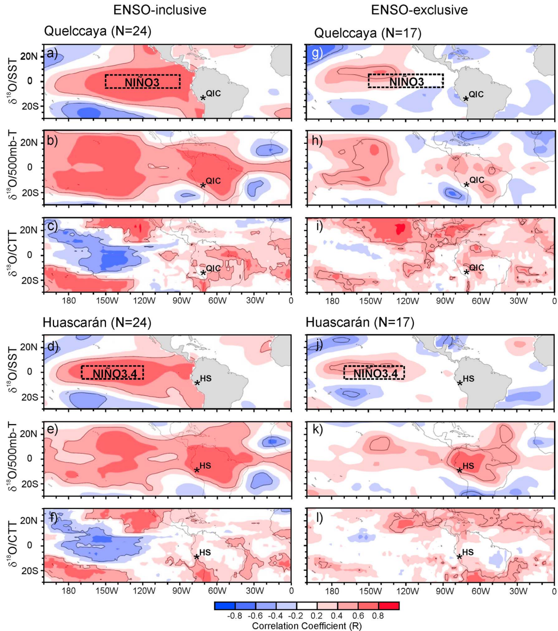
Figure 6. Pearson two-tailed correlation ( R ) fields between QIC TY1 \delta^{18}\text{O} (between 1973/1974 and 2015/2016) and (a) DJF SSTs (Huang et al., 2015; Liu et al., 2015), (b) DJF 500 mb-T (Kalnay et al., 1996), and (c) DJF CTTs (Kalnay et al., 1996). (d–f) Same as in Figures 6a–6c but for HS TY \delta^{18}\text{O} (1973/1974 to 1992/1993, 2012/2013 to 2015/2016). (g–i) Same as in Figures 6a–6c but with ENSO events of -1.0 > \text{ONI} > +1.0 excluded. (j–l) Same as for Figures 6d–6f but with ENSO events of -1.0 > \text{ONI} > +1.0 excluded. Red shading indicates positive R , blue shading indicates negative R , and black contours denote R values with significance levels ( p ) = 0.05.
