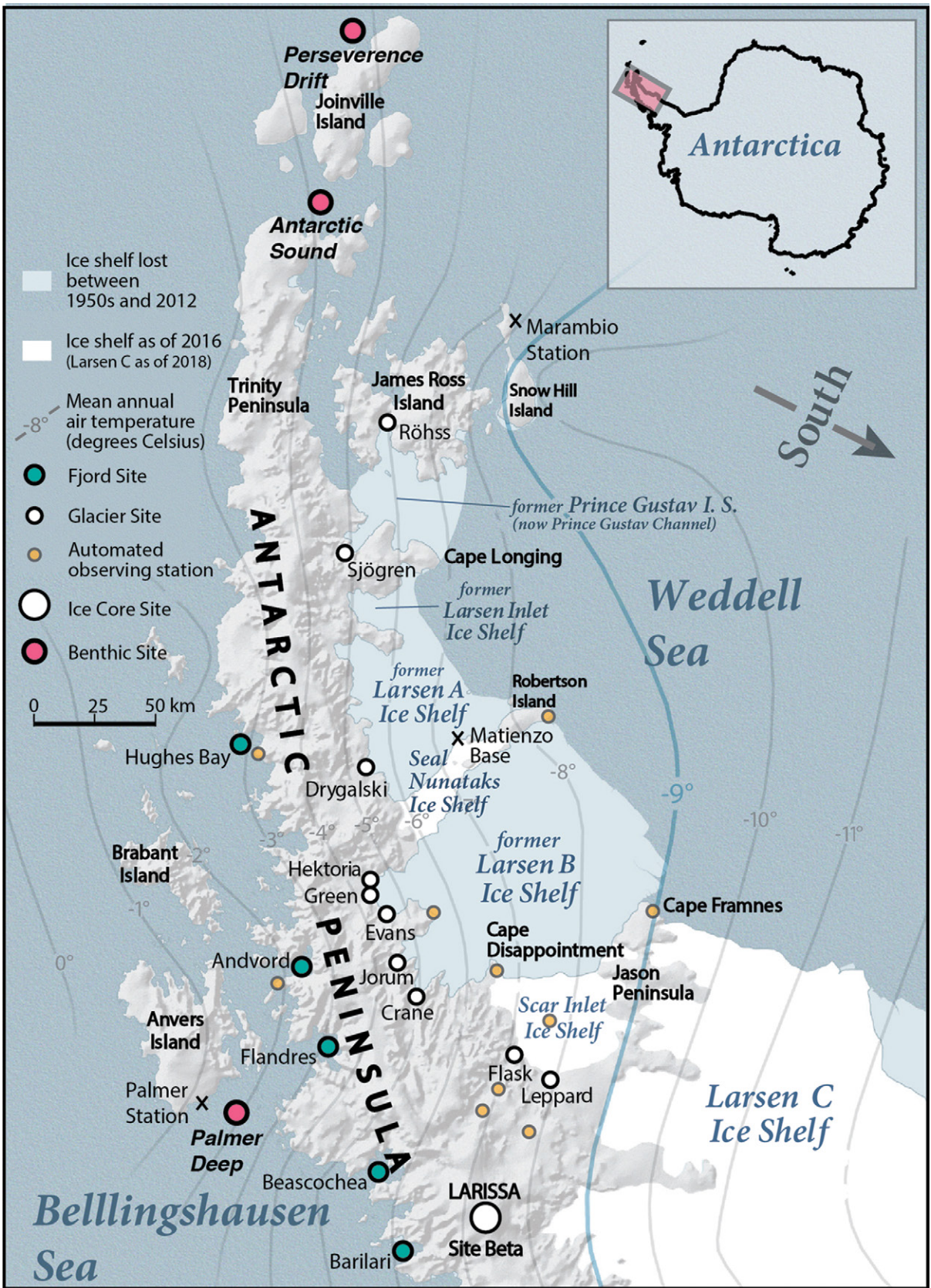
Figure 3. LARISSA study region and sites of research focus. Geographic features highlighted by circles were areas of detailed investigations or instrumentation in support of regional characteristics. Contours are isotherms of mean annual temperature at sea level; -9^{\circ}\text{C} has been suggested as the limit of long-term ice-shelf stability in previous studies. Base map provided with permission from XNR/Terra Carta ( www.terracarta.com ).
