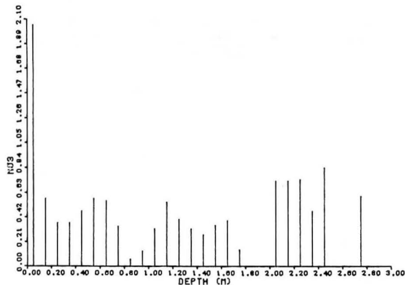
Fig. 2 Concentrations in \mu\text{M} of sulfate, nitrate-plus-nitrite and nitrate plotted against depth in snow-pit #1, Quelccaya ice cap.
