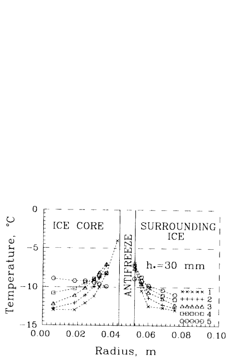
Fig. 2. Temperature distribution in the ice core during ATED drilling; 1-5: t=10, 40, 80, 120, and 440 s.
