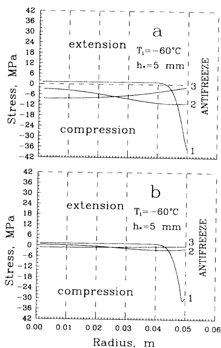
Fig. 3. Maximum axial stress in an ice core during (a) ATED and (b) m-ATED drilling (1-3: t=5, 310 and 605 s).
